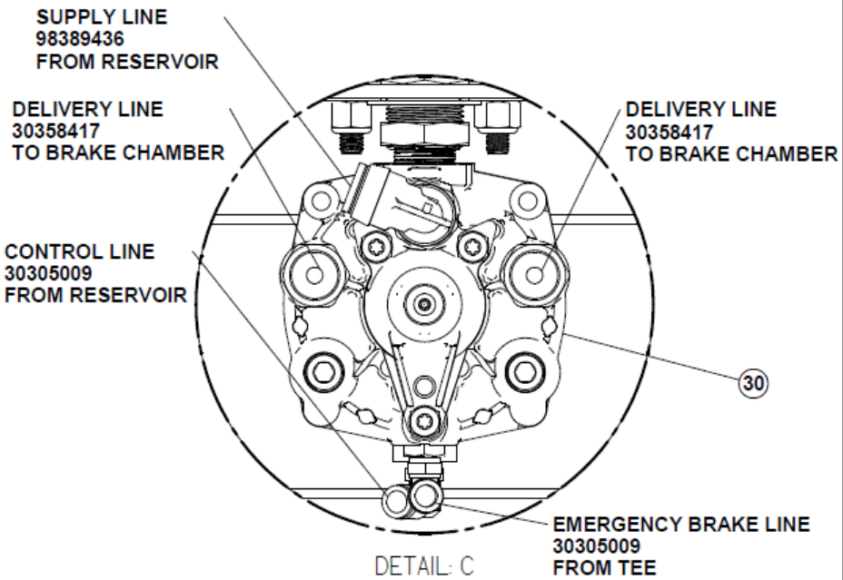
FRAME END VIEW BOOSTER HIDDEN FOR CLAIRITY
